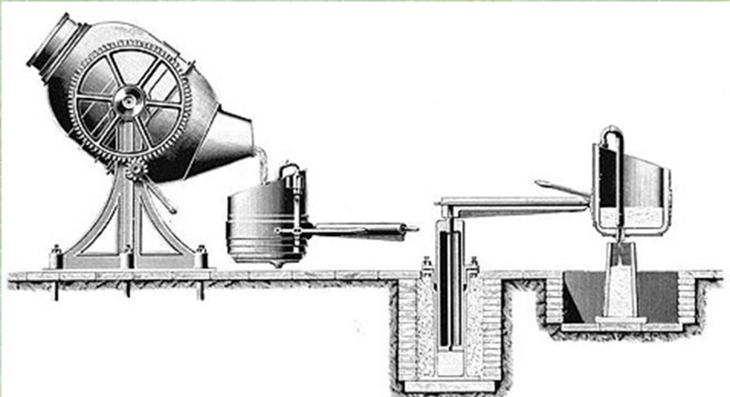
FIG. 11. EARLY FORM OF BESSEMER CONVERTING PLANT AT SHEFFIELD
